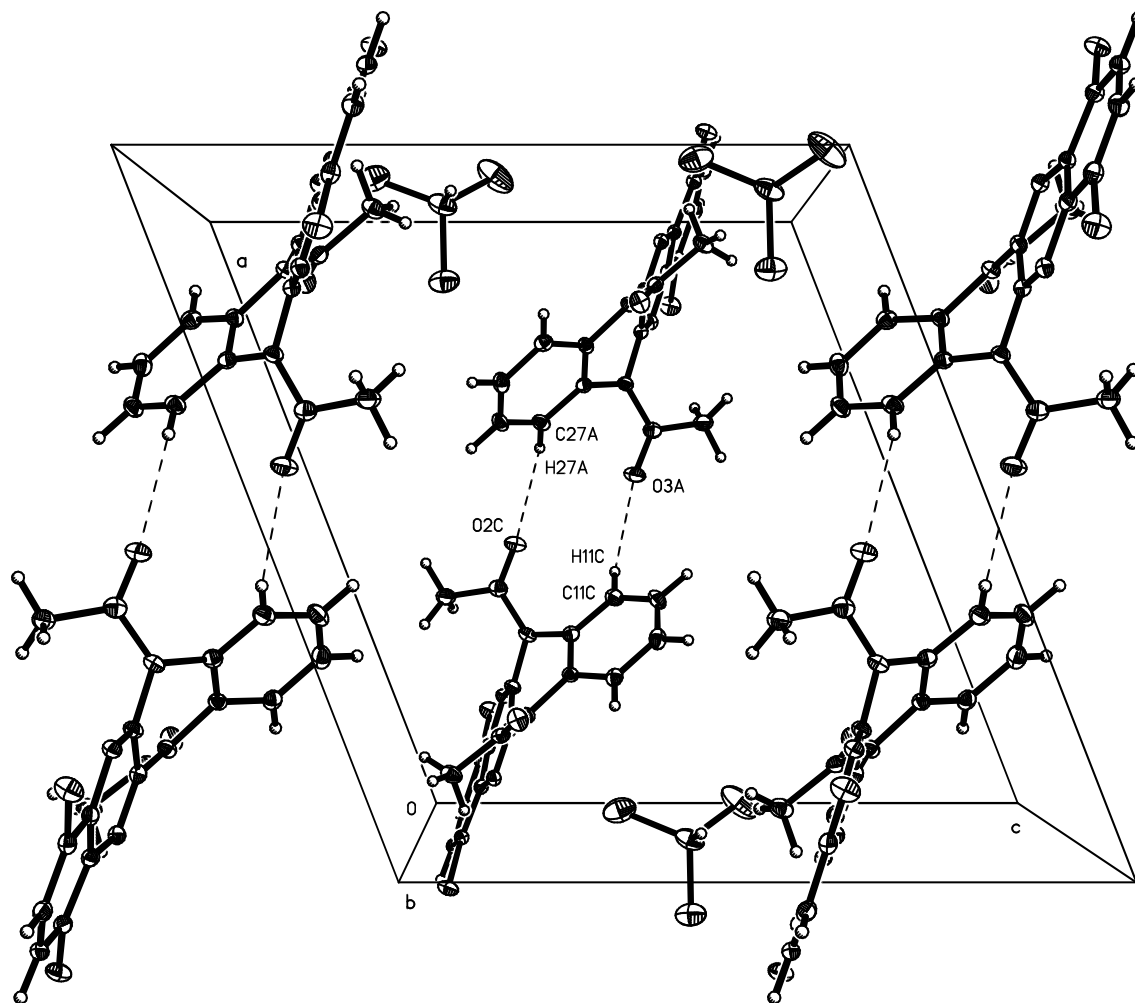
Figure 4. A perspective of the crystal packing of 9 , showing the hydrogen interactions.
