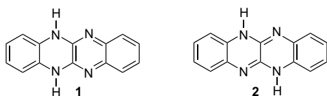
Figure 1. The structures of isomeric fluo flavines.
