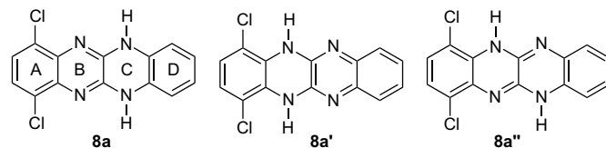
Figure 2. The structures of isomeric dichlorofluoquinolines.
