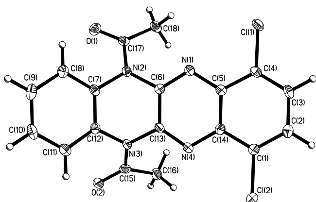
Figure 3. ORTEP of 9 , with thermal ellipsoids shown at 50% probability.
